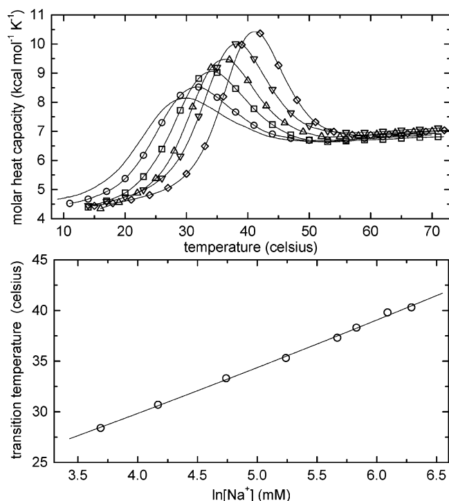
FIGURE 5: Stability of \alpha S55D/E59D as a function of \text{Na}^+ concentration. (A) DSC data are shown for experiments conducted at total \text{Na}^+ concentrations of 65 (no symbol), 190 (○), 290 (□), 340 (△), 440 (▽), and 540 mM (◇). All of the scans were performed at a protein concentration between 7.0 and 7.4 mg/mL. (B) Stoichiometry of \text{Na}^+ binding. The melting temperature is plotted as a function of the natural logarithm of the \text{Na}^+ concentration (in millimolar). The solid line indicates the best fit to a second-order polynomial. The slope of the curve when \ln[\text{Na}^+] = 5.29 , corresponding to 200 mM \text{Na}^+ , was used to calculate the stoichiometry of \text{Na}^+ binding, as described in the text.
